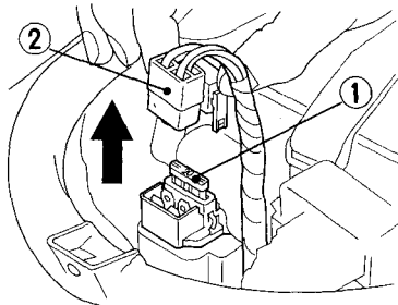
(1) Main fuse
