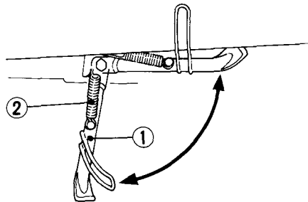
(1) Side stand
